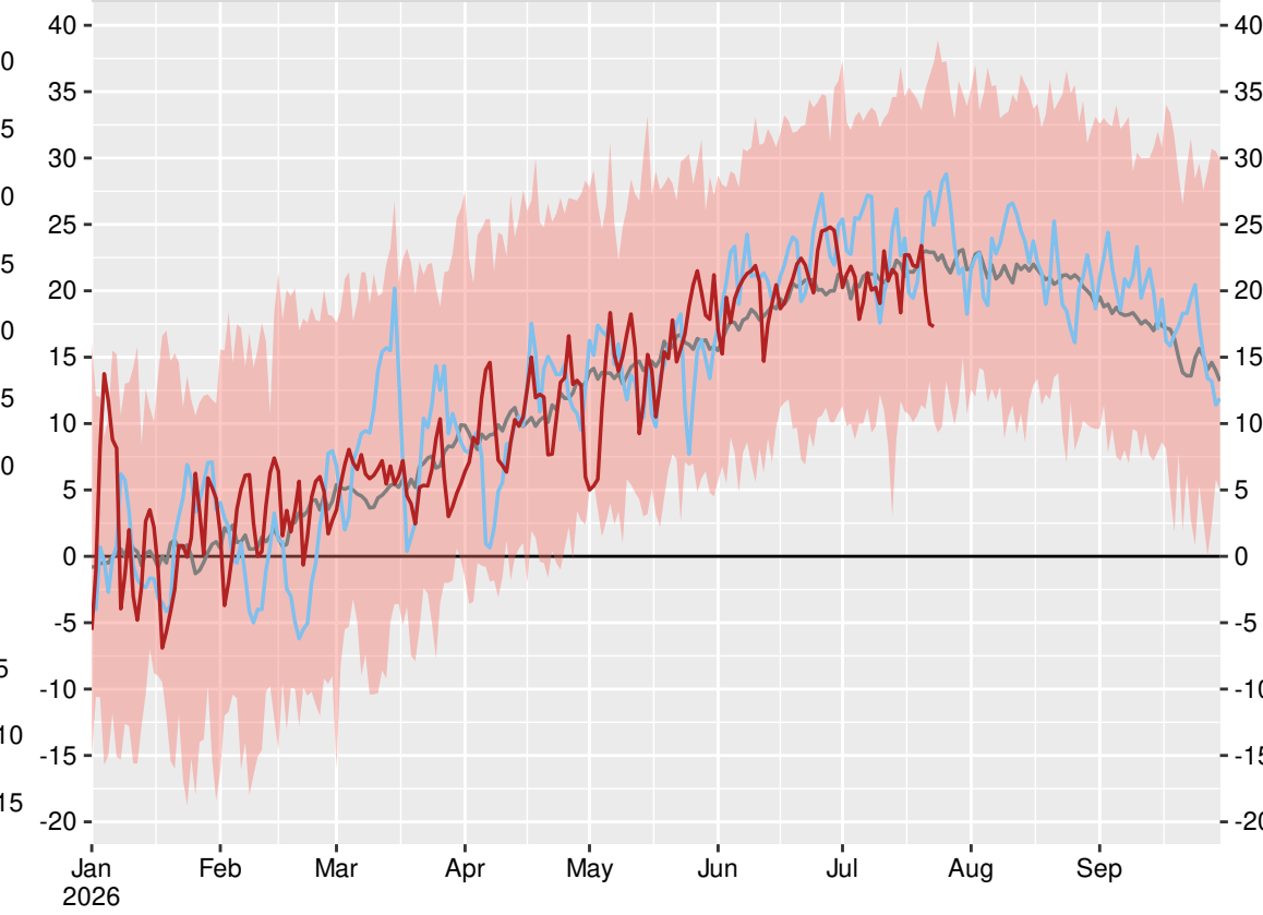
София (15614), 2026-07-23
