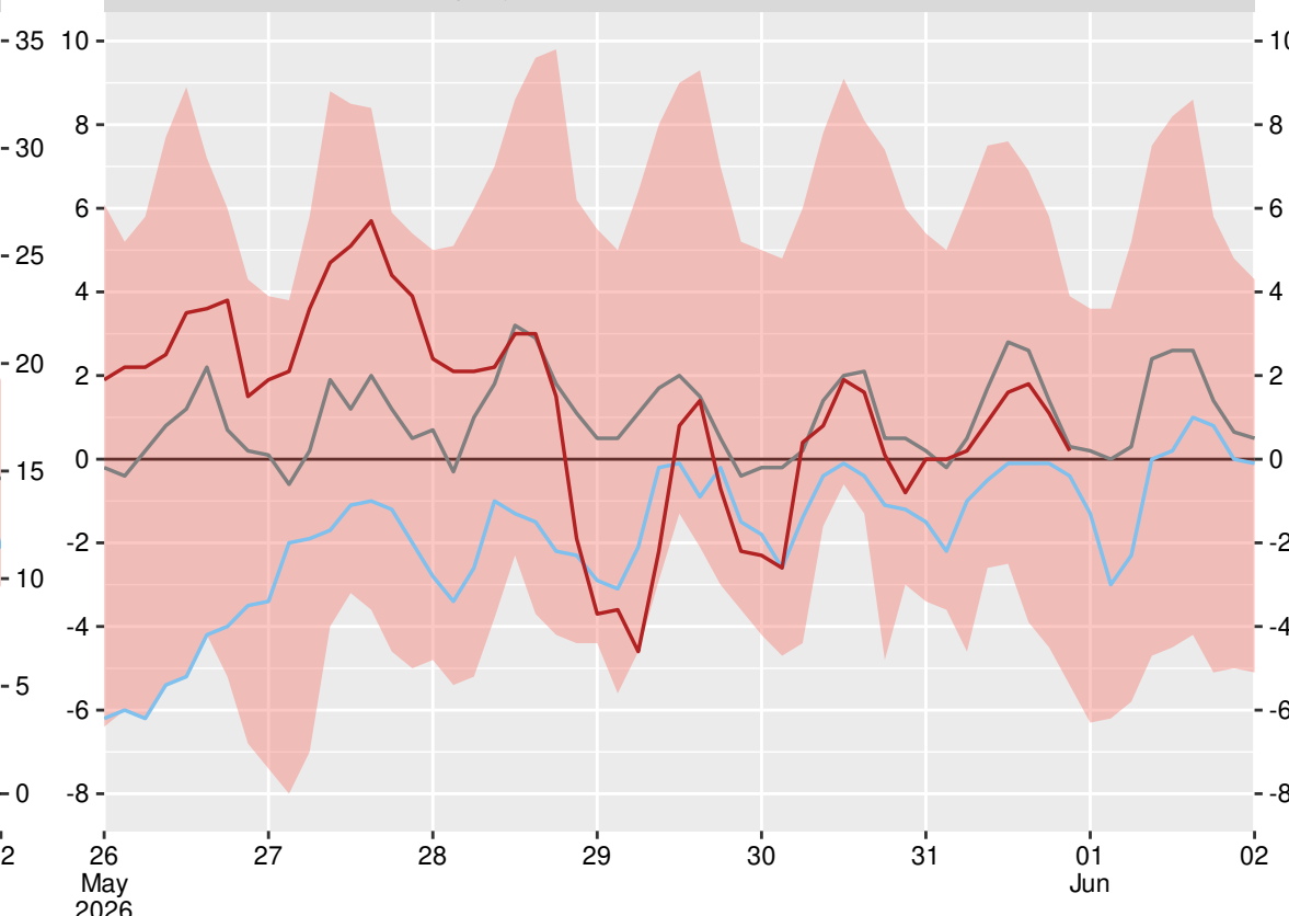
Ловеч (15525), 2026-05-31 21:00:00
