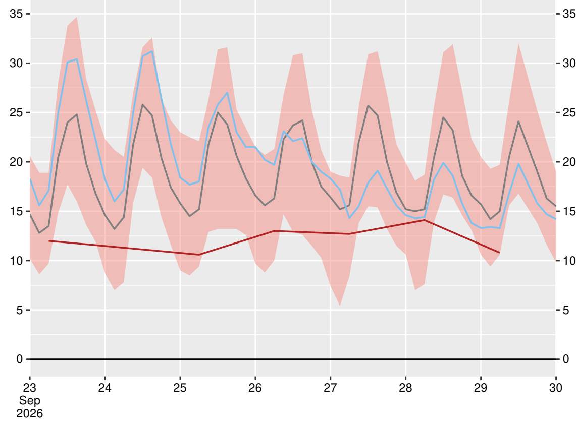
София (15614), 2026-09-29 06:00:00
