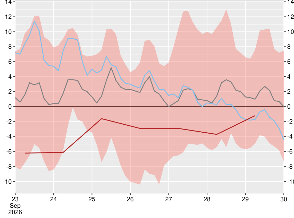
Ловеч (15525), 2026-09-29 06:00:00
