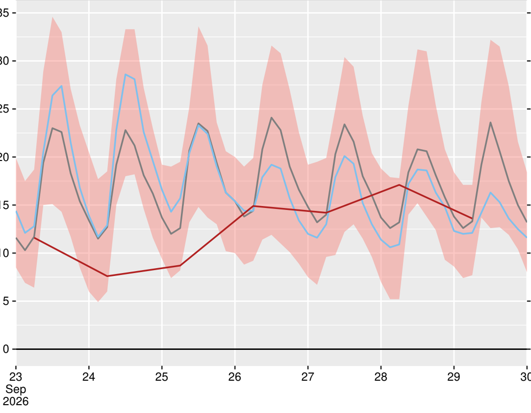
Разград (15549), 2026-09-29 06:00:00
