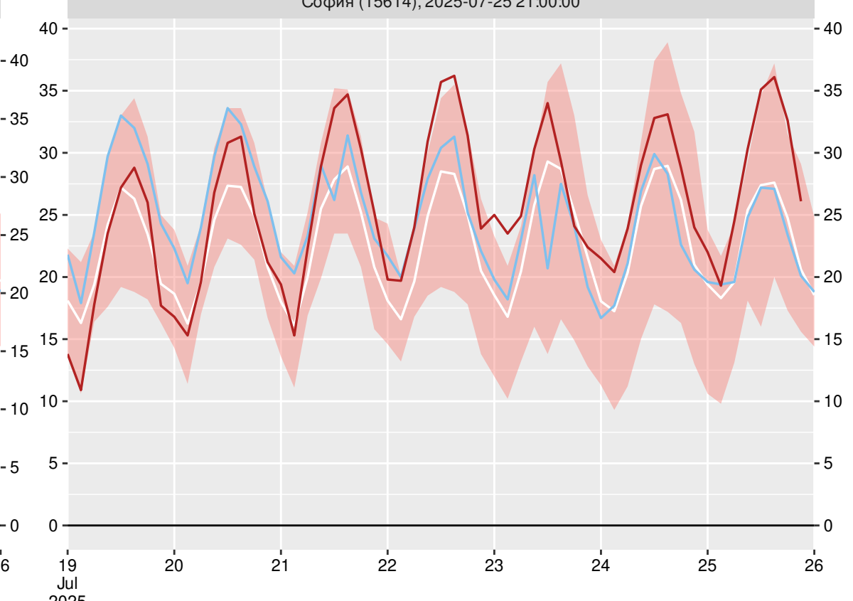
София (15614), 2025-07-25 21:00:00
