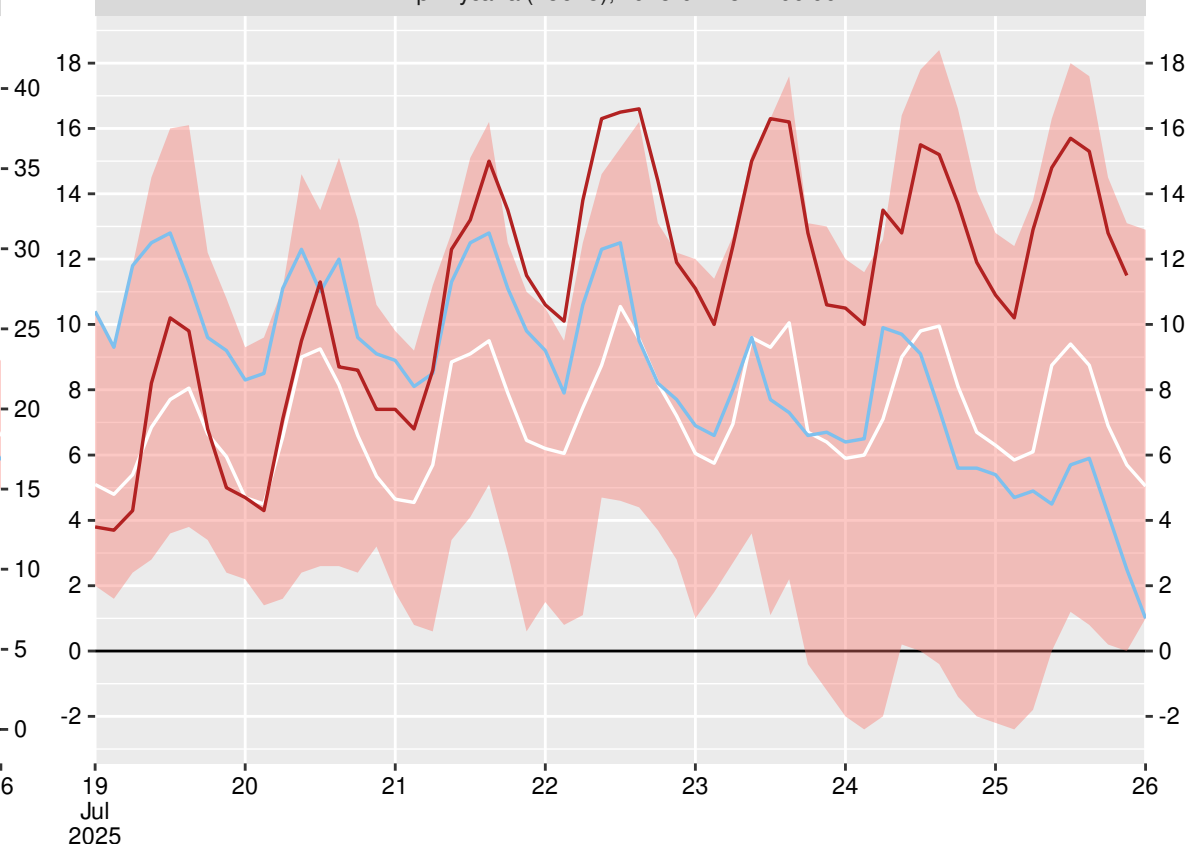
Ловеч (15525), 2025-07-25 21:00:00
