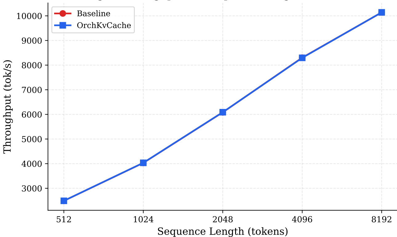
Fig.1: Throughput vs. Sequence Length (batch=4)
