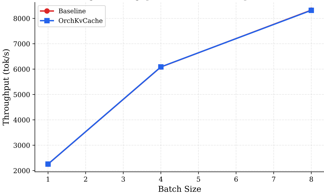
Fig.2: Throughput vs. Batch Size (seq=2048)
