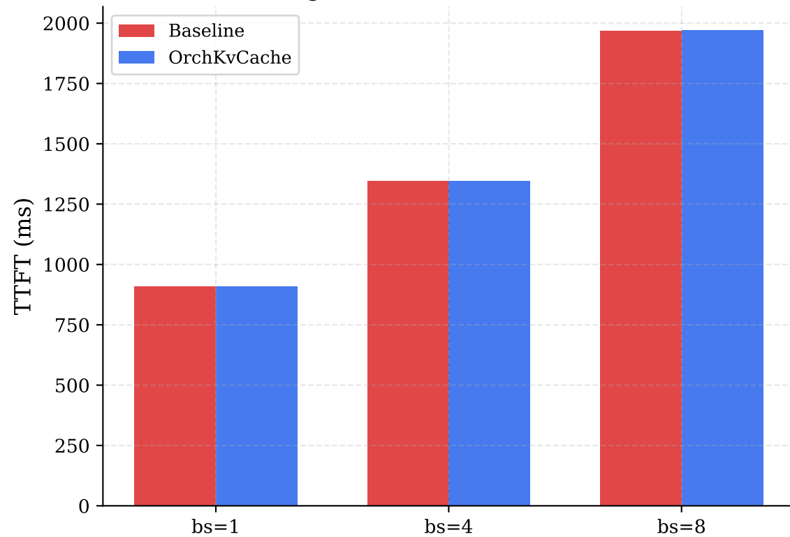
Fig.3a: Time-to-First-Token
