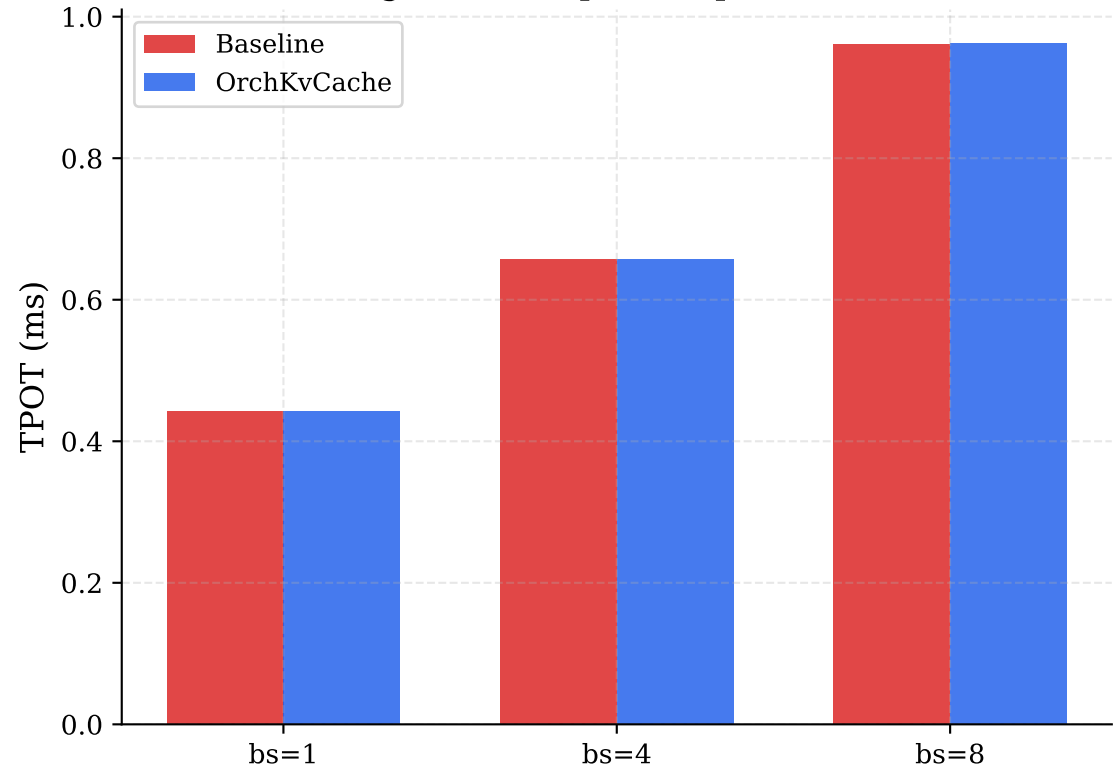
Fig.3b: Time-per-Output-Token
