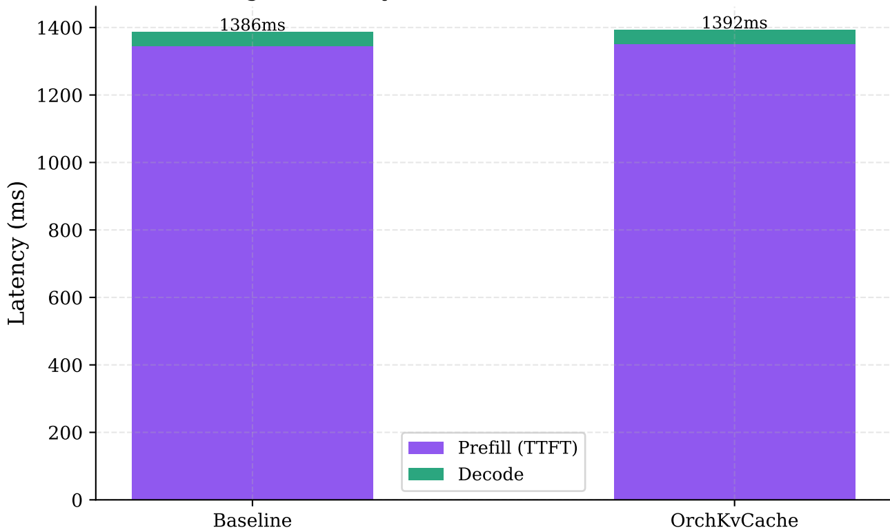
Fig.5: Latency Breakdown (Prefill + Decode)
