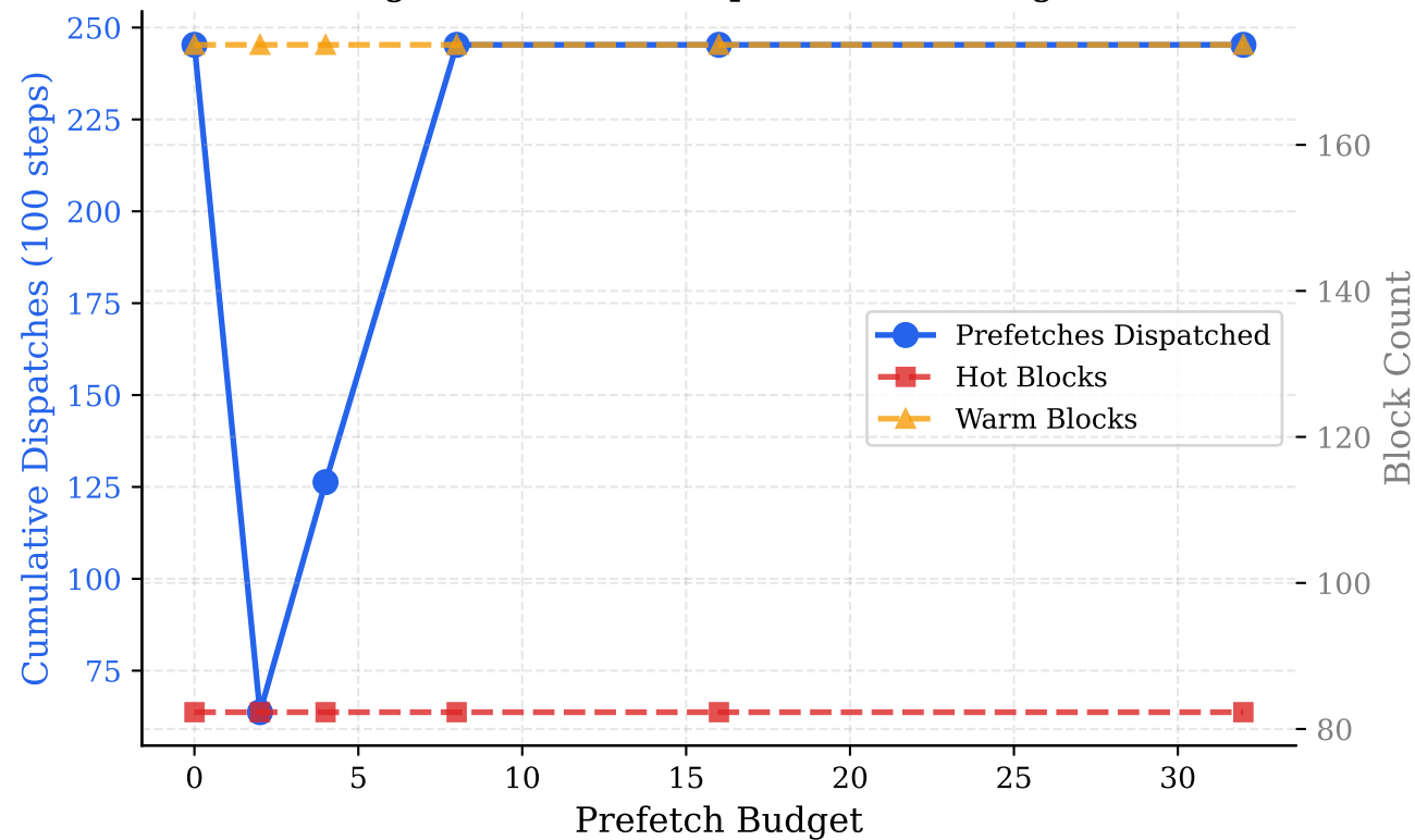
Fig.11: Prefetch Dispatches vs. Budget
