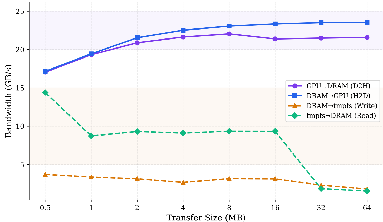
Fig.13: Storage Tier Bandwidth (A100-SXM4 + DDR4 + tmpfs)
