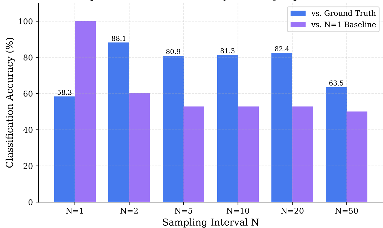
Fig.16: Classification Quality vs. Sampling Interval
