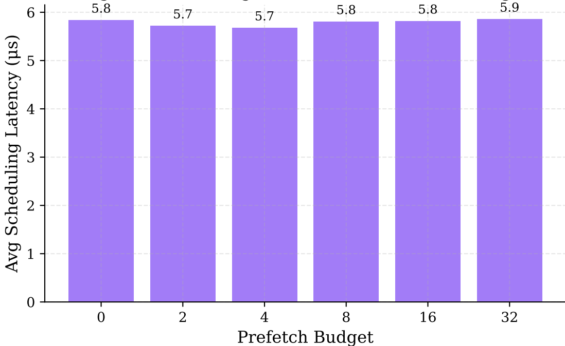
Fig.12: Scheduling Overhead vs. Prefetch Budget
