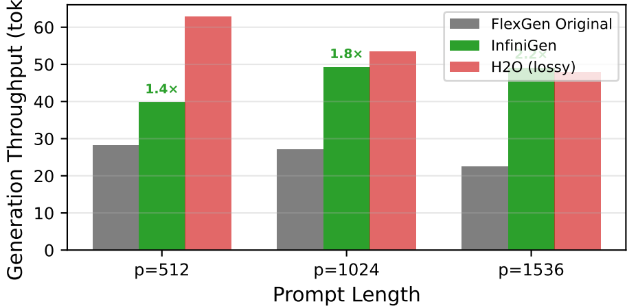
OPT-1.3B (FlexGen offloading, bs=4, gen=128)
