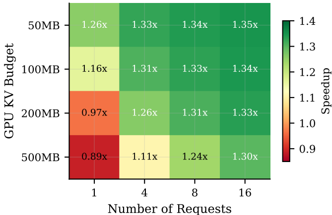
OrchKv/Naive Speedup, seq=4096
