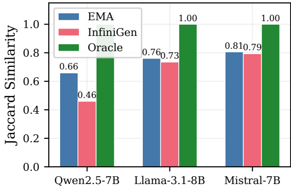
Predictor Accuracy Comparison
