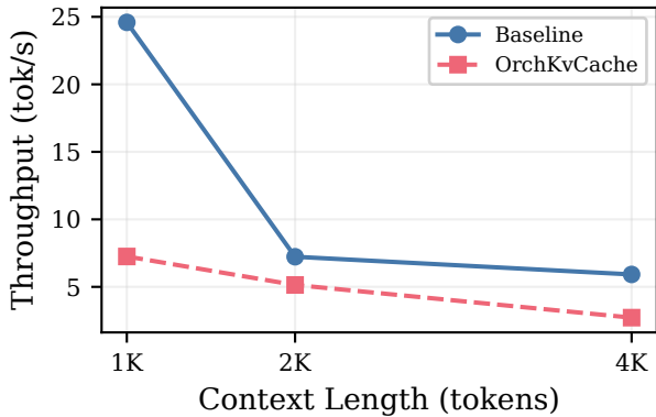
(a) Throughput vs Context Length
