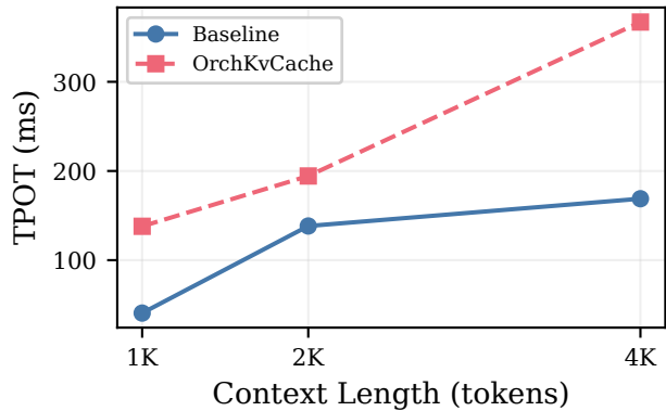
(b) TPOT vs Context Length
