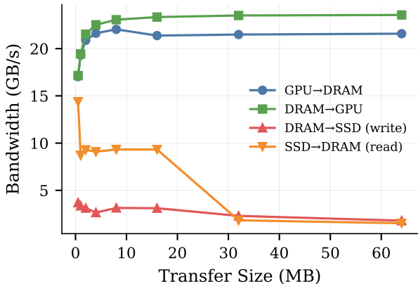
Inter-Tier Bandwidth (E8)
