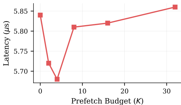
(b) Per-Step Overhead (E7)
