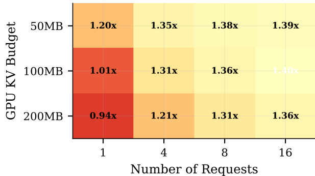
(a) Qwen2.5-7B
