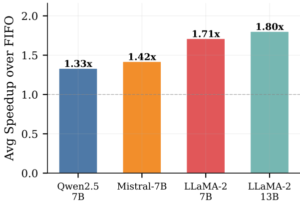
OrchKvCache vs FIFO, budget=50MB, seq=2048
