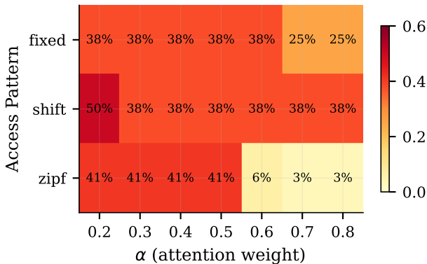
Hot Ratio by Policy Weight (E5)
