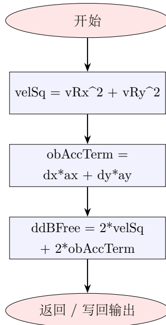
图 1: computeBarrierSecondDerivativeFree 函数程序流程图
