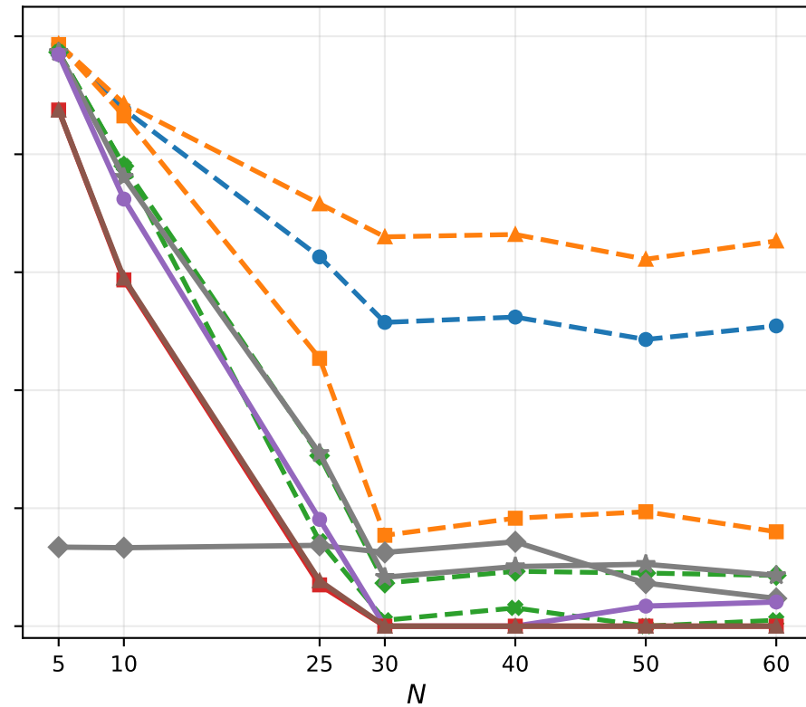
DeepSeek-Reasoner
