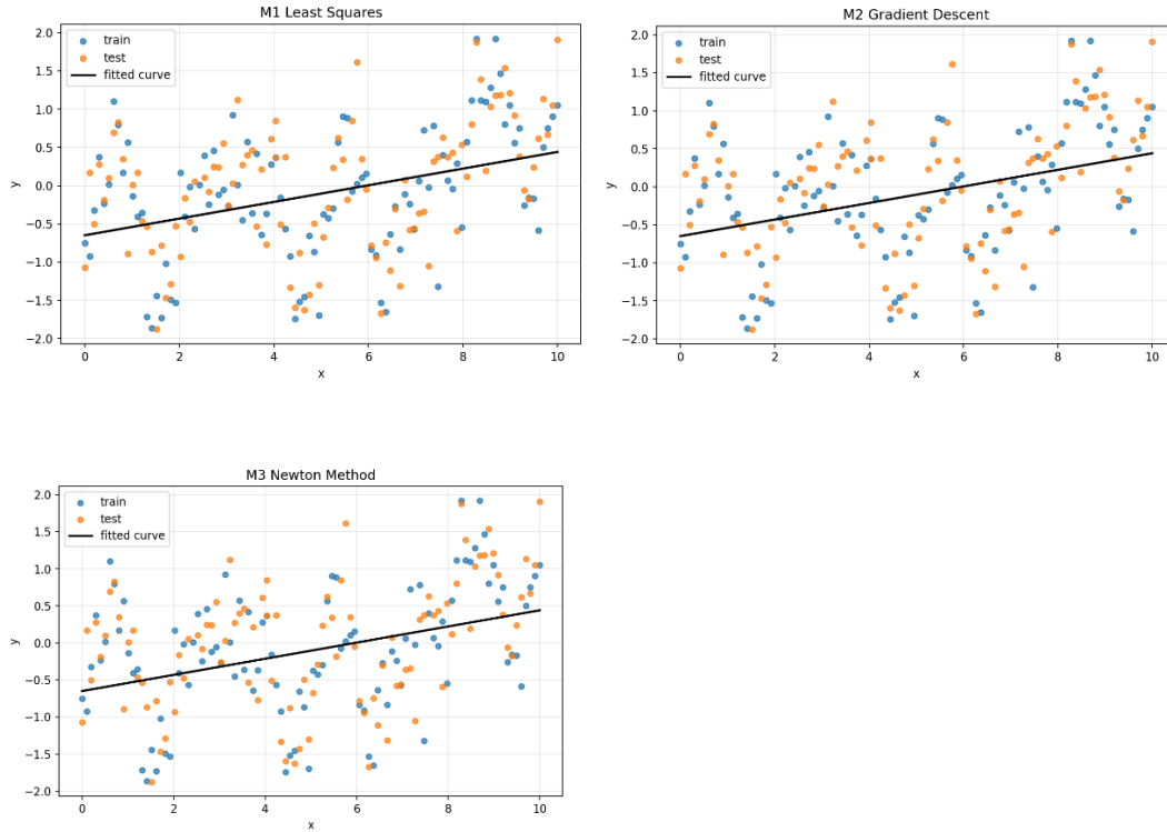
Figure 2: Visualization of linear regression fits
