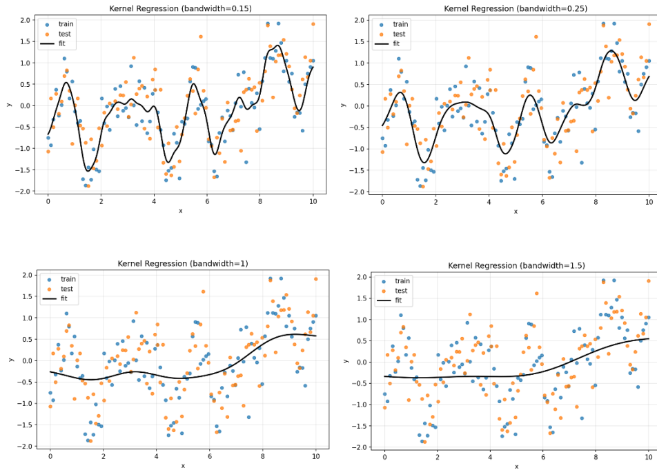
Figure 5: Kernel regression fits for different bandwidth values
