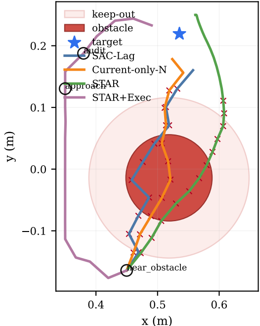
(b) Top-down gripper trajectory
