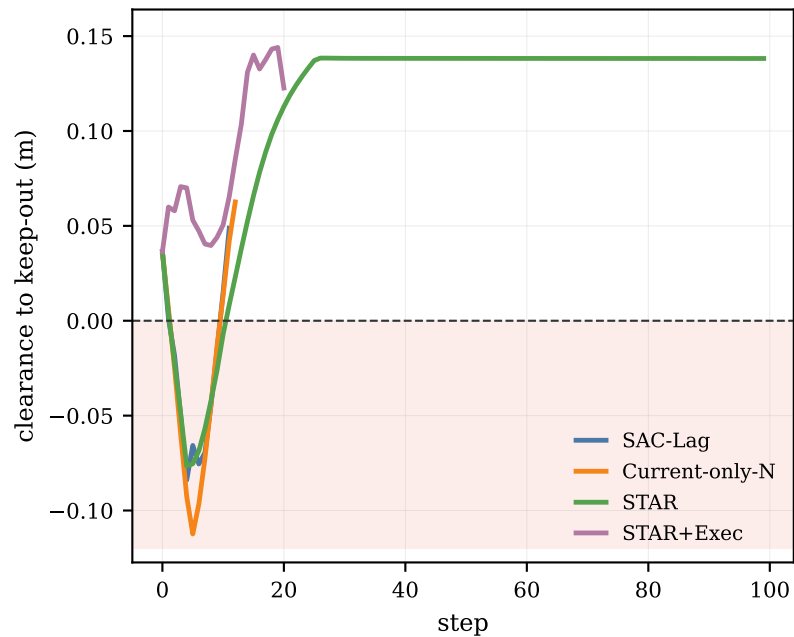
(c) Clearance profile
