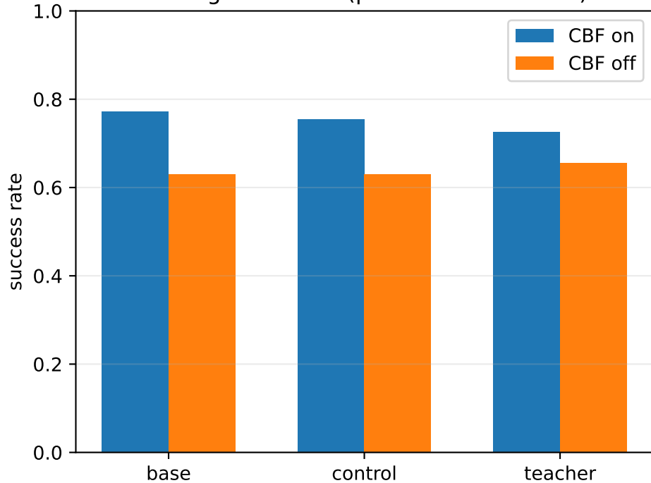
F1 target success (partial formal result)
