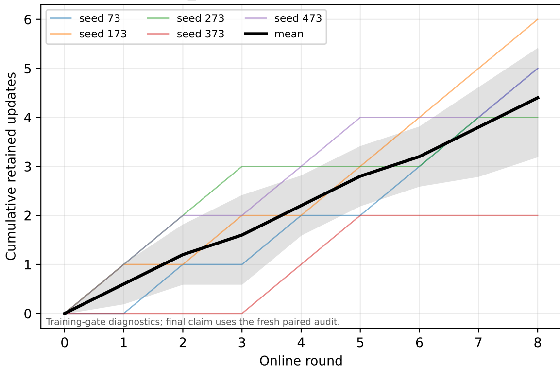
contact_stability: retained-update trajectory
