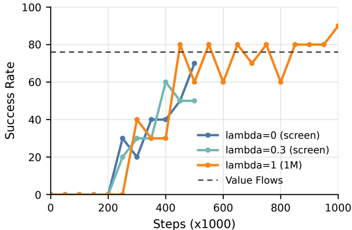
Cube-double task2
