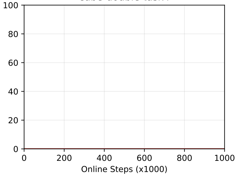
cube-double task4
