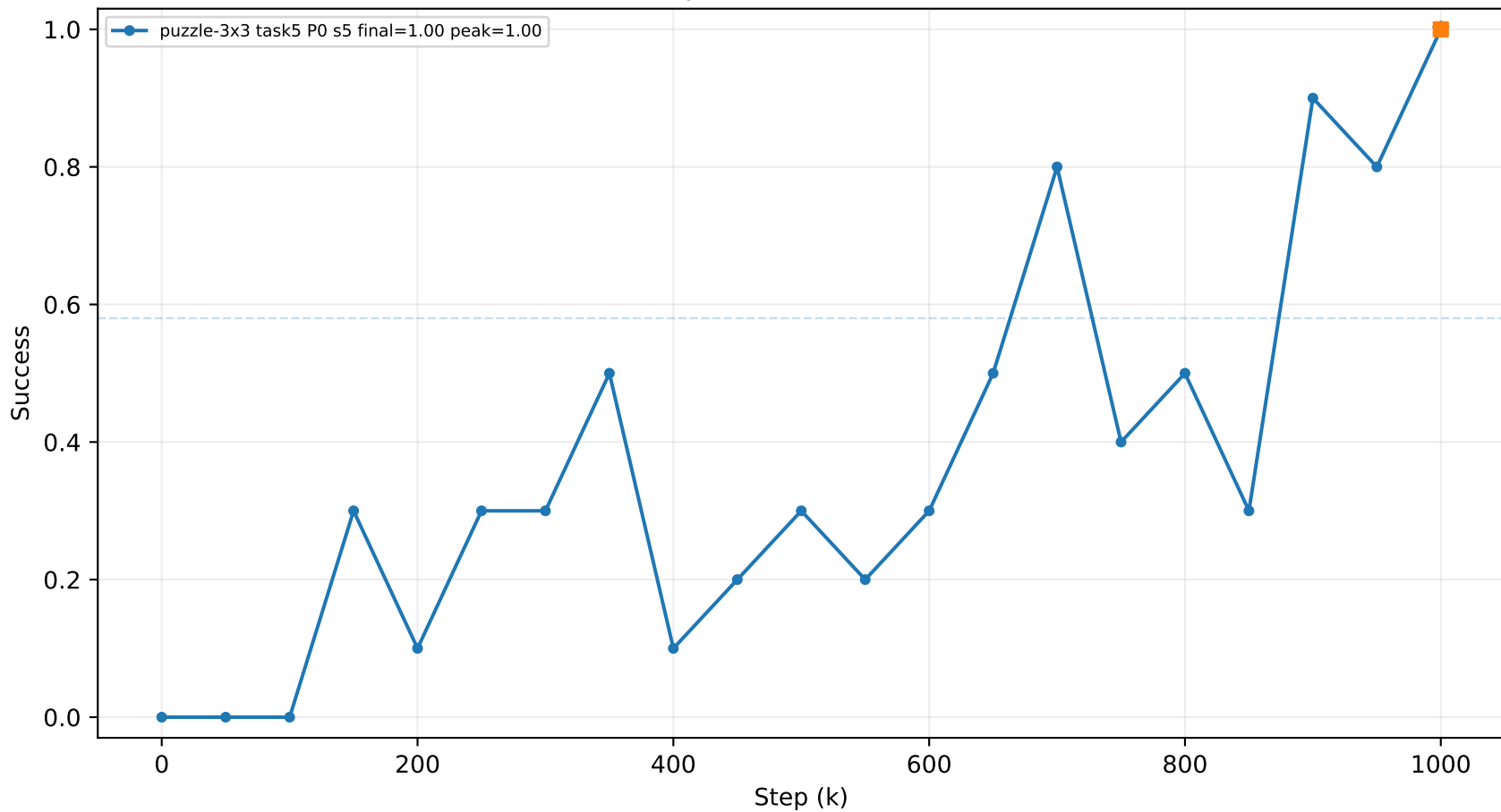
puzzle3x3 task5
