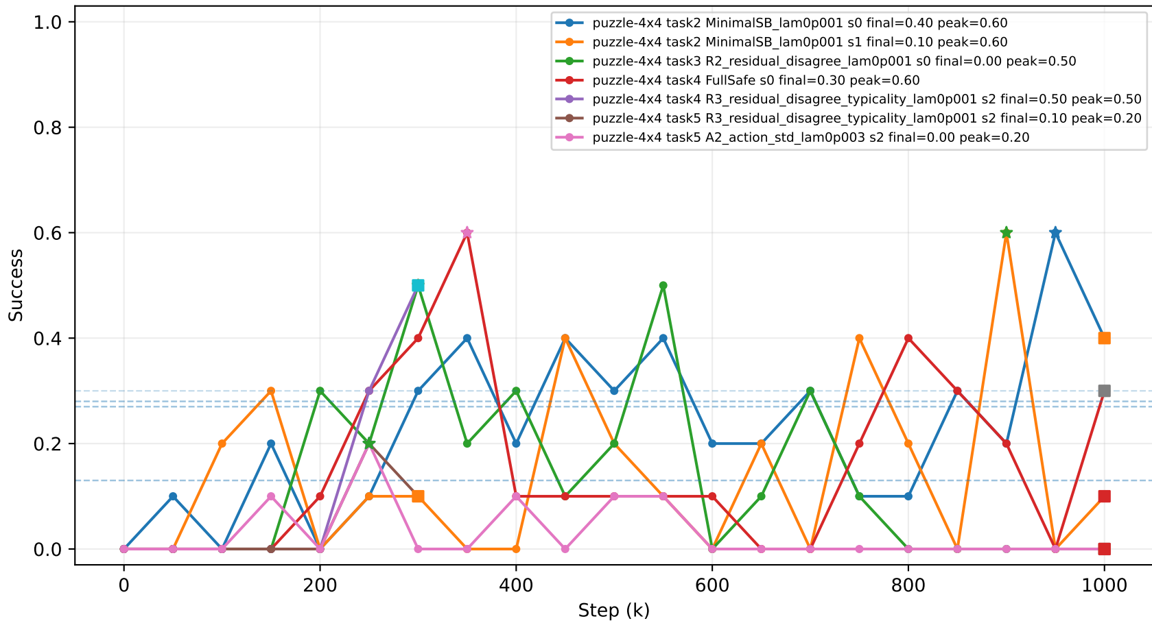
puzzle4x4 all tasks
