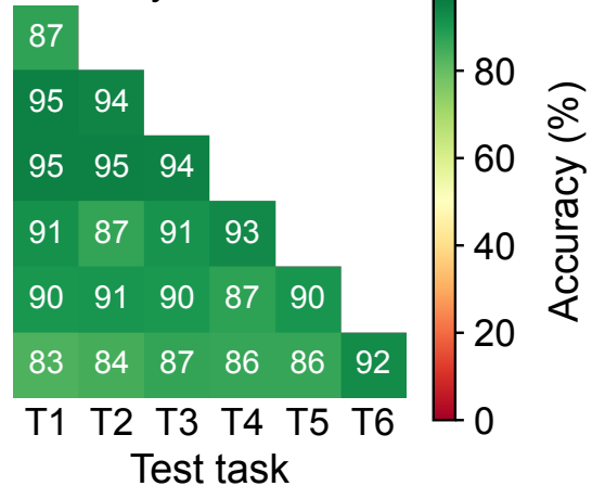
DynDFCL
