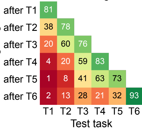
FedAvg
