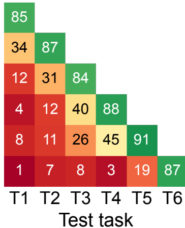
DCFCL
