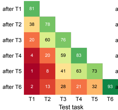
FedAvg
