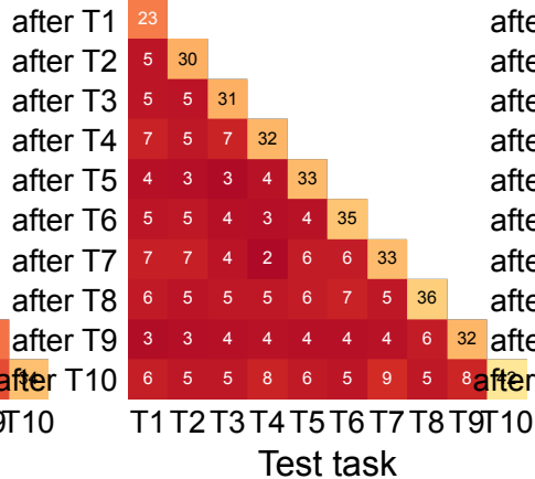
DCFCL
