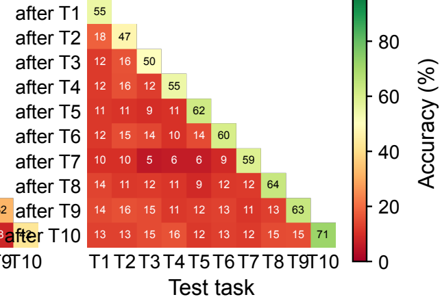
CollEdge
