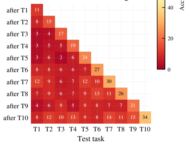
CIFAR-100 — FedAvg
