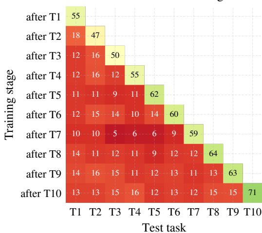
CIFAR-100 — CollEdge
