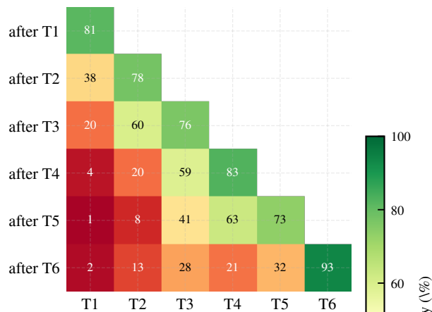
CIFAR-100 — FedAvg
