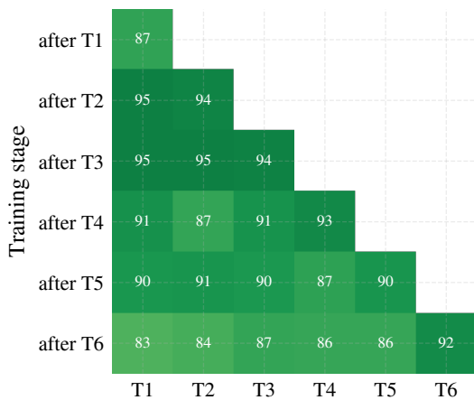
CIFAR-100 — CollEdge
