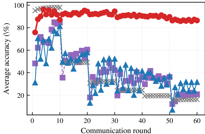
EMNIST-Letters
