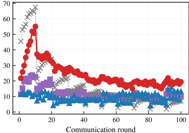
CIFAR-100
