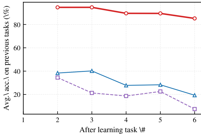
EMNIST-Letters
