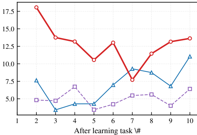
CIFAR-100
