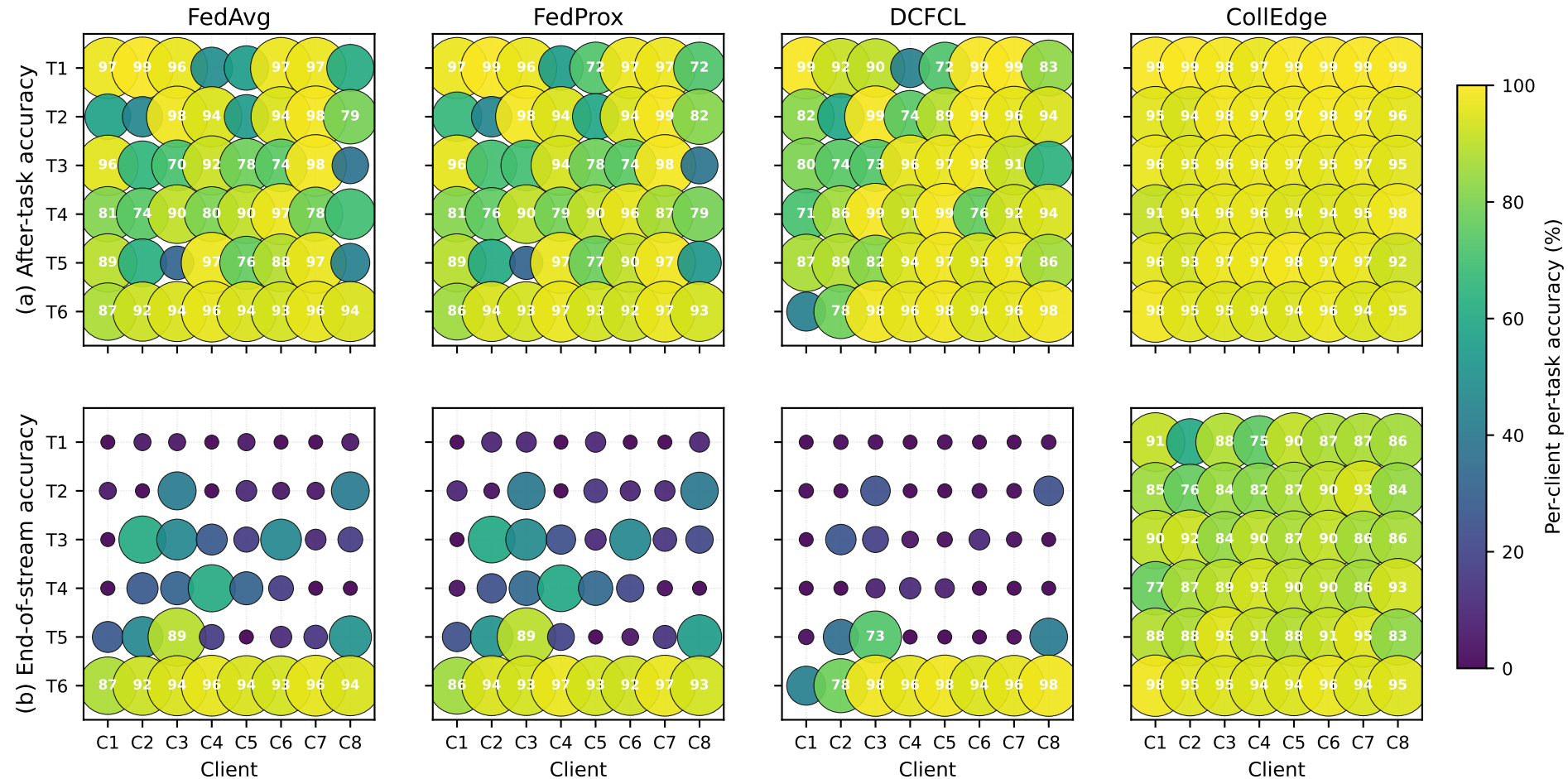
Client x Task accuracy on EMNIST-Letters: after-task (top) vs. end-of-stream (bottom)
