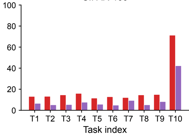
CIFAR-100
