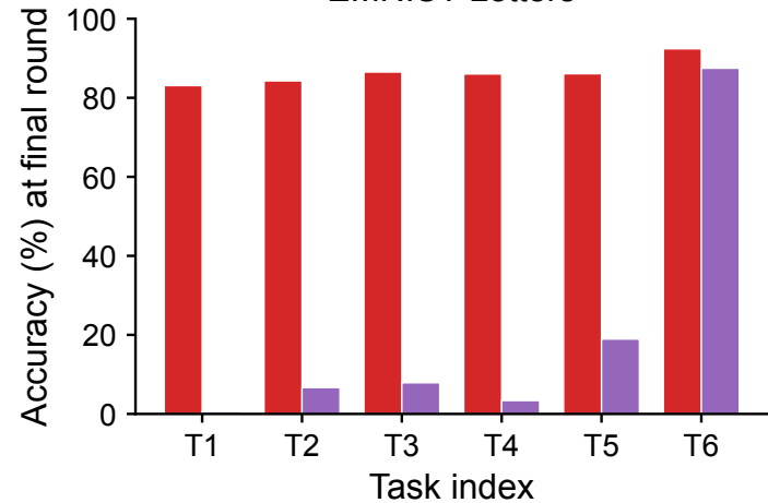
EMNIST-Letters
