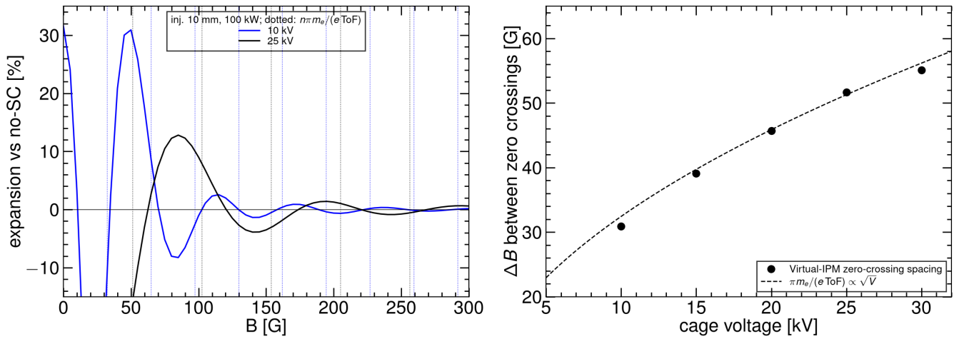
Figure 3. Left: Fine C expansion vs B at 10 and 25 kV (100 kW) with the predicted zeros n \cdot \pi m_e / (e \cdot \text{ToF}) as dotted lines. Right: spacing between zero crossings vs cage voltage against \pi m_e / (e \cdot \text{ToF}) \propto \sqrt{V} .
