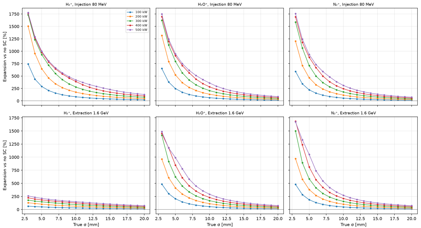
Figure 3. Expansion vs true \sigma_x at 0.1 T for 100–500 kW. Smaller beams and higher power give dramatically larger expansion; injection is worse than extraction for \text{H}_2^+ , but \text{H}_2\text{O}^+ and \text{N}_2^+ can be worse at extraction (longer ToF).
