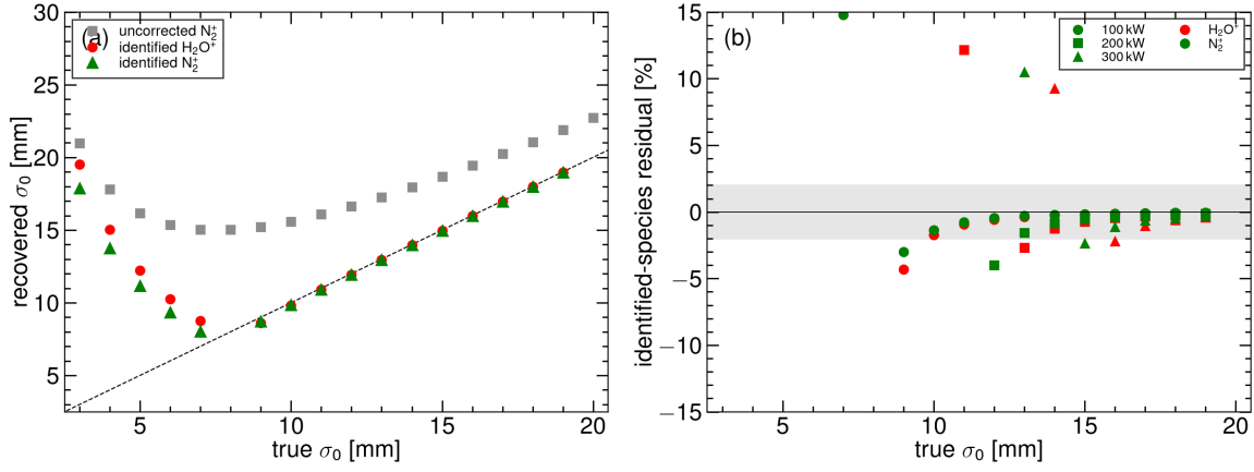
Fig. 13: (a) Injection 100 kW: uncorrected N_2^+ \sigma_m and the identified H_2O^+ and N_2^+ inverts versus true \sigma_0 (leave-one-out). (b) Identified-species residual at 100–300 kW. Red: H_2O^+ . Green: N_2^+ . The grey band is \pm 2\% . Open markers are wall-clipped families.
