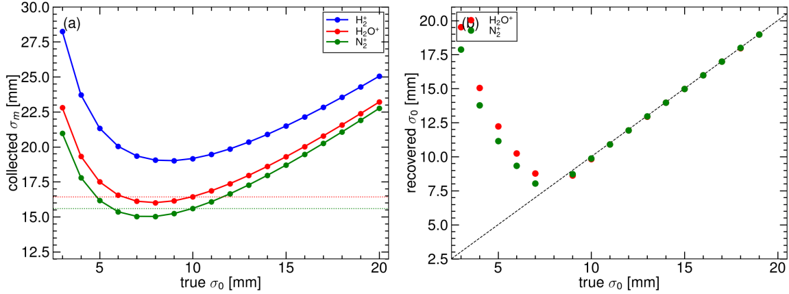
Fig. 12: Injection, 100 kW, 25 kV, B = 0 . (a) Collected \sigma_m versus true \sigma_0 . Dotted lines are the H_2O^+ and N_2^+ widths of a 10 mm beam (16.44 and 15.60 mm). (b) Leave-one-out invert of the identified H_2O^+ or N_2^+ table on \sigma_0 \geq \sigma_0^* . Empty markers at \sigma_0 < 8 mm have no root on that branch.
