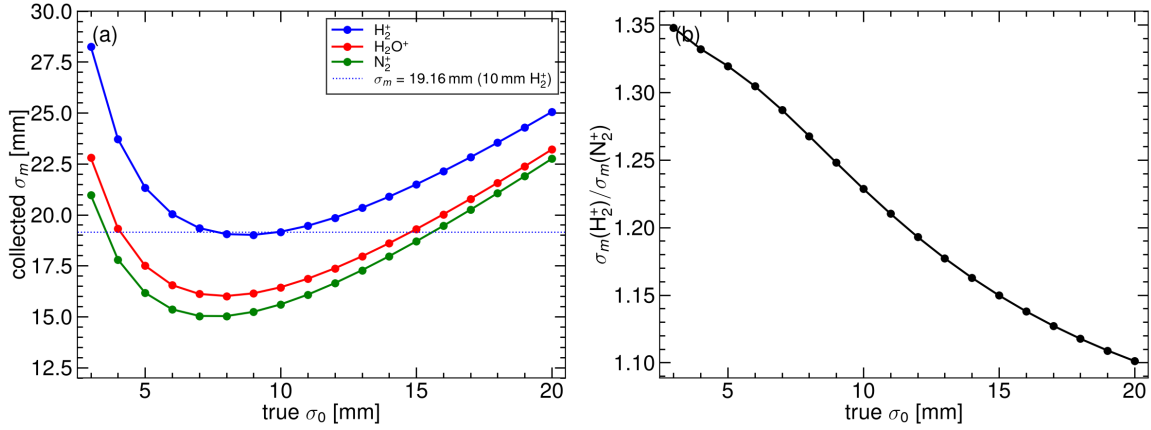
Fig. 12: Injection, 100 kW, 25 kV, B = 0 . (a) Collected \sigma_m versus true \sigma_0 . The dotted line is the \text{H}_2^+ width of a 10 mm beam (19.16 mm); it cuts the \text{H}_2^+ curve twice. (b) Ratio \sigma_m(\text{H}_2^+)/\sigma_m(\text{N}_2^+) , monotonic in \sigma_0 .
