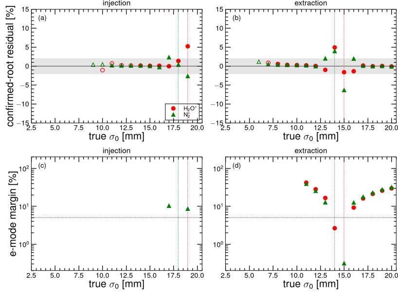
Fig. 17: As Fig. 14, at 500 kW.
