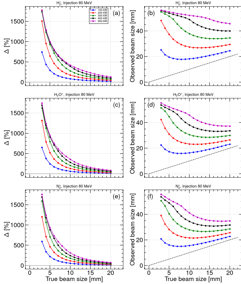
Fig. 3: Injection, 80 MeV, 0.1 T, 25 kV. Left column: ion-mode expansion \Delta versus true size \sigma_0 for 100–500 kW; right column: observed width \sigma_m versus \sigma_0 for the same points, one row per species. The dashed line is \sigma_m = \sigma_0 . The 3 mm/500 kW family saturates on the cage wall ( \sigma_m \approx 56 mm).
