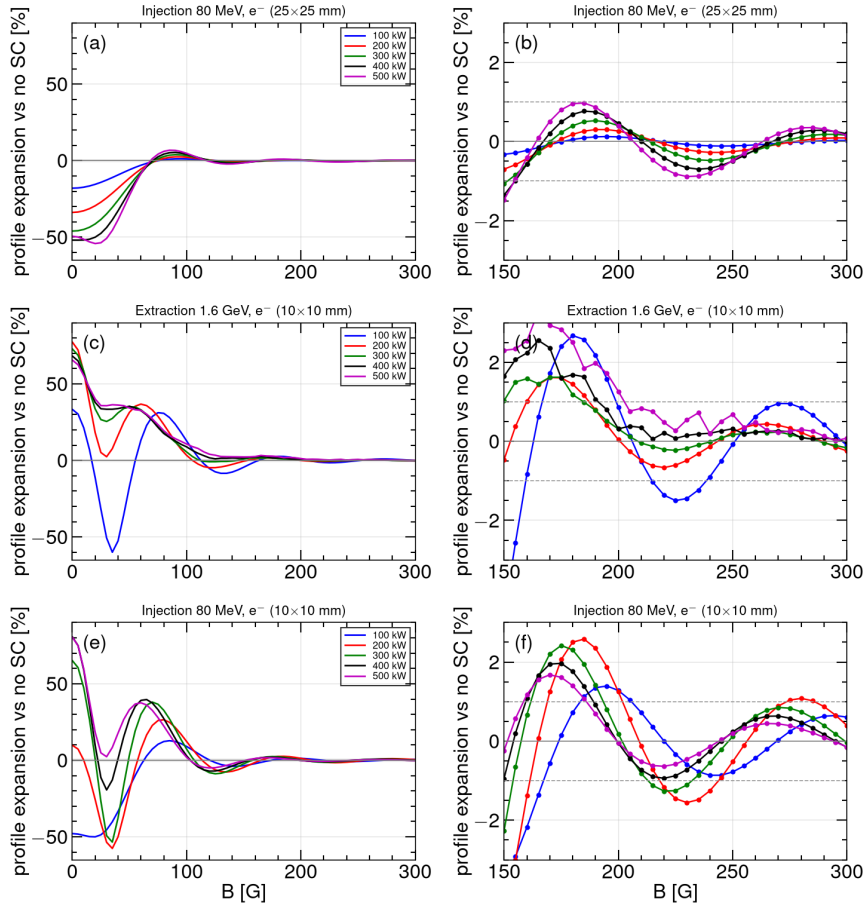
Fig. 6: Electron-mode expansion versus guiding field for painted injection (25 mm; a, b), extraction (10 mm; c, d) and the 10 mm injection core (e, f), at 100–500 kW. Left: 0–300 G, the grey band is \pm 1\% . Right: 150–300 G on a \pm 3\% scale, dashed lines at \pm 1\% . At 300 G every family lies inside \pm 1\% .
