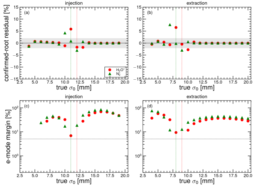
Fig. 15: As Fig. 14, at 200 kW.
