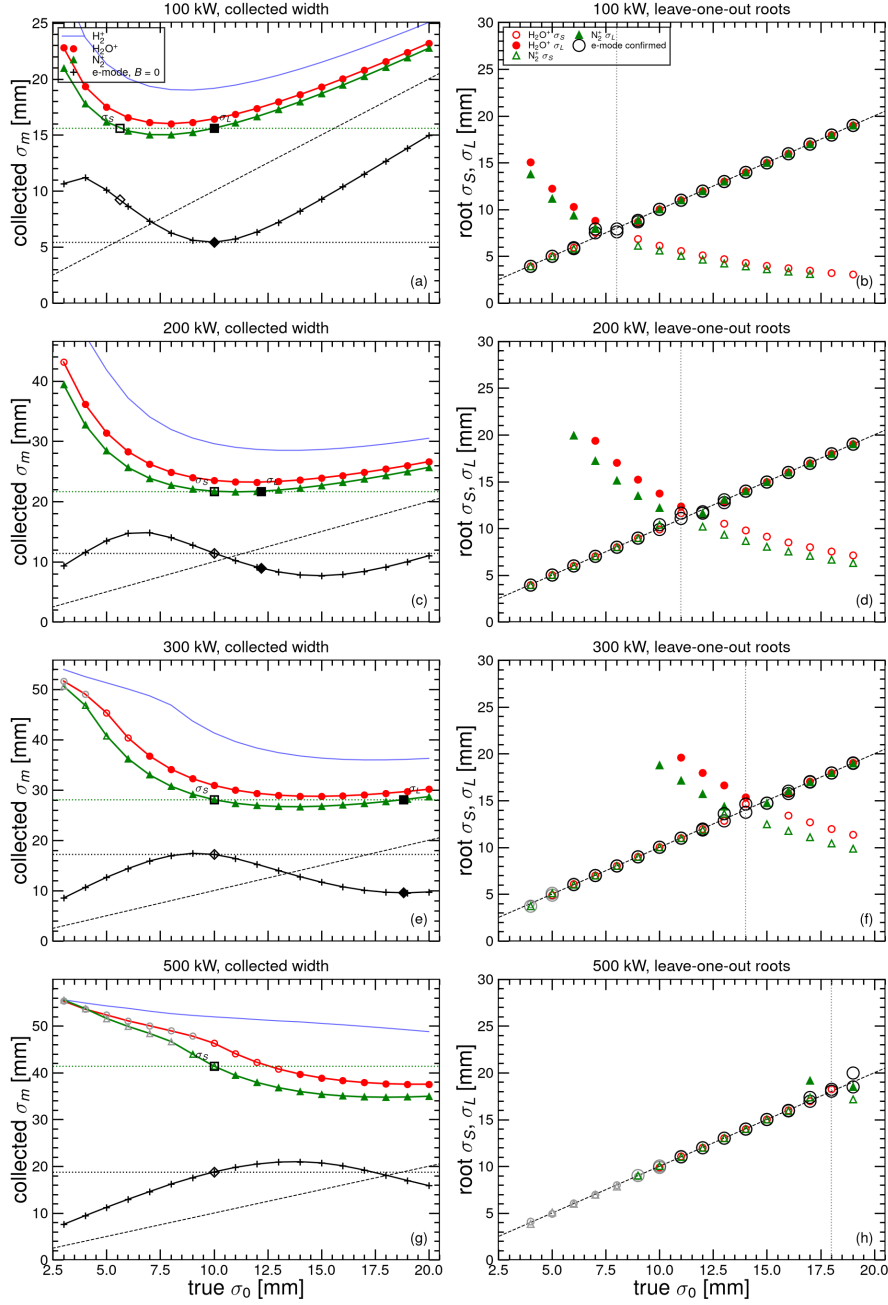
Fig. 12: Injection, 80 MeV, 25 kV, B = 0 , one row per power (100, 200, 300, 500 kW). Left: collected \sigma_m of \text{H}_2\text{O}^+ (red) and \text{N}_2^+ (green) versus true \sigma_0 ; thin blue is \text{H}_2^+ ; the black curve is the electron width at B = 0 ; the dashed line is \sigma_m = \sigma_0 . Open coloured markers are collected in full but above 40 mm; grey markers lose ions on the cage. The green dotted line is the \text{N}_2^+ width of a 10 mm beam with its two roots \sigma_S (open square) and \sigma_L (filled square); the black dotted line is the electron width of the same beam, and the diamonds are the electron widths the two roots predict, T_e(\sigma_S) (open) and T_e(\sigma_L) (filled)—the one on the dotted line is the consistent root. Right: leave-one-out roots \sigma_S (open) and \sigma_L (filled) for both species; the black ring marks the root confirmed by the electron width; the dotted vertical is the \text{N}_2^+ fold.
