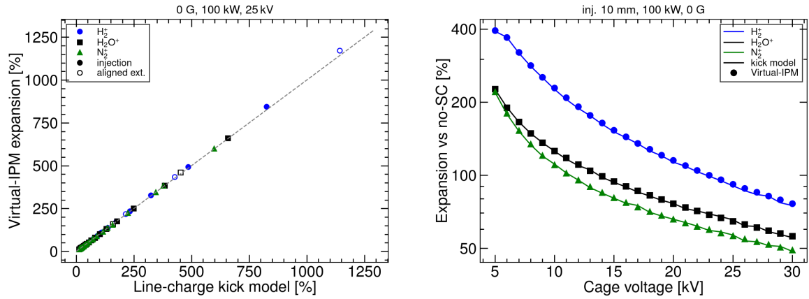
Fig. 5: Left: ion-mode expansion at 0 G, 100 kW and 25 kV, reduced kick model versus Virtual-IPM. Filled markers: injection \sigma_0 = 3\text{--}20 mm. Open markers: extraction (3, 5, 7, 10, 15, 20 mm). Right: expansion versus cage voltage, injection 10 mm. Curves: kick model. Markers: Virtual-IPM. Agreement is \pm 1\% absolute on the left and \leq 4\% relative on the right.
