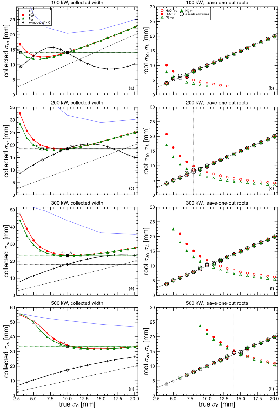
Fig. 13: As Fig. 12 for extraction (1.6 GeV, \beta = 0.929 , \sigma_t = 20 ns, ions generated in time with the bunch), 25 kV, B = 0 . The thin blue H_2^+ curve is tabulated on a coarser size grid.
