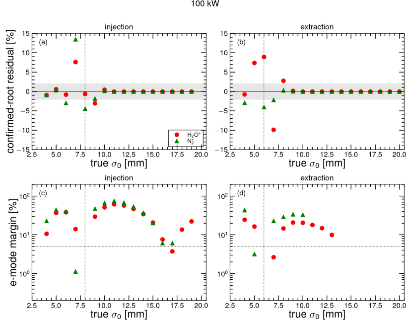
Fig. 14: 100 kW, B = 0 , 25 kV. (a, b) Residual of the root confirmed by the B = 0 electron width versus true \sigma_0 (leave-one-out, interior of the table, ions inside the cage) at injection and extraction. Red circles: \text{H}_2\text{O}^+ ; green triangles: \text{N}_2^+ ; open markers are collected above 40 mm; the grey band is \pm 2\% ; dotted verticals are the folds \sigma_0^* of the two species. (c, d) Electron margin |T_e(\sigma_S) - T_e(\sigma_L)|/\sigma_e at the points with two roots inside the tables; the dotted horizontal is 5%.
