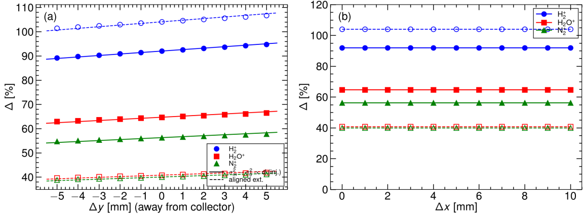
Fig. 11: Ion-mode closed-orbit offset at B = 0 , 10 mm, 100 kW, 25 kV. (a) \Delta versus vertical offset \Delta y . Filled: injection. Open: extraction. Lines: \sigma_m^2 - \sigma_0^2 \propto d . (b) \Delta versus horizontal offset \Delta x ; the width is translation-invariant.
