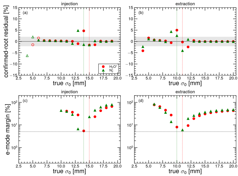
Fig. 16: As Fig. 14, at 300 kW.
