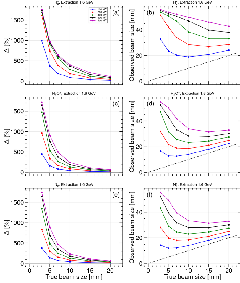
Fig. 4: As Fig. 3 for extraction (1.6 GeV), with the ions generated in time with the bunch.
