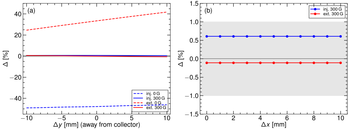
Fig. 10: Electron-mode closed-orbit offset, 10 mm beams, 100 kW. (a) \Delta versus vertical offset \Delta y . Dashed: B = 0 . Solid: 300 G. The grey band is \pm 1\% . (b) \Delta versus horizontal offset \Delta x at 300 G.
