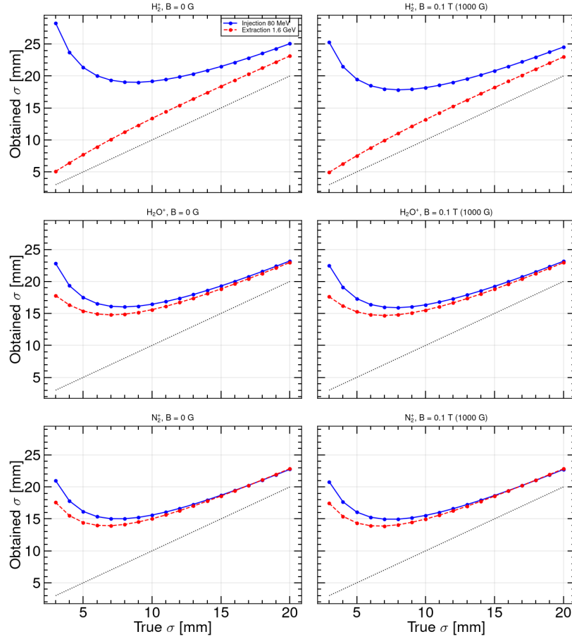
Fig. 2: Ion-mode obtained width \sigma_m versus true width \sigma_0 at 100 kW for the three species (rows) at B = 0 (left) and 0.1 T (right). The dotted line is \sigma_m = \sigma_0 . Space charge inflates every point; the guiding field does not change the ion image.
