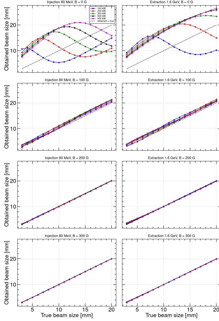
Fig. 8: Electron-mode obtained width versus true width at B = 0, 100, 200 and 300 G (rows) at injection (left) and extraction (right), 100–500 kW. From 200 G the points lie on the diagonal except at 3 mm.
