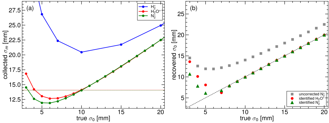
Fig. 14: Aligned extraction, 100 kW, 25 kV, B = 0 , 1.6 GeV. (a) Collected \sigma_m versus true \sigma_0 on the 1 mm I2 grid. Dotted lines are the H_2O^+ and N_2^+ widths of a 10 mm beam (14.11 and 14.03 mm). H_2^+ is the coarse I1 curve. (b) Leave-one-out invert of the identified H_2O^+ or N_2^+ table on \sigma_0 \geq \sigma_0^* . Grey squares: uncorrected N_2^+ \sigma_m .
