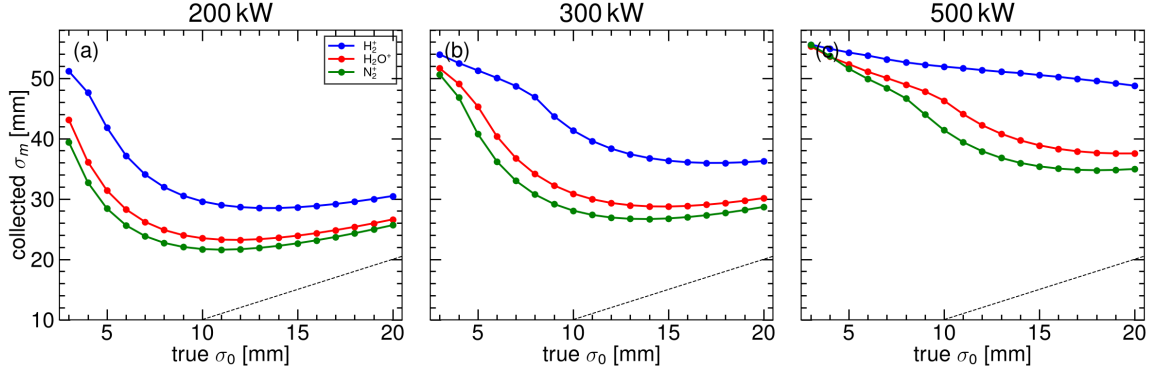
Fig. 14: Injection, 25 kV, B = 0 , 80 MeV. Collected \sigma_m versus true \sigma_0 at 200, 300 and 500 kW. The dashed line is \sigma_m = \sigma_0 . The minimum moves out with power; at 500 kW the heavies sit against the cage wall.
