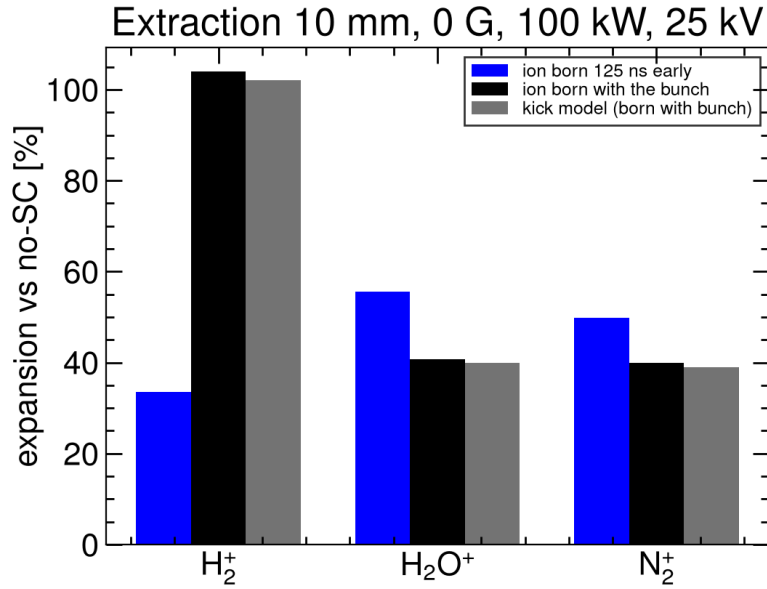
Fig. 17: Extraction, 10 mm, 0 G, 100 kW, 25 kV. Virtual-IPM with the ion born in time with the bunch matches the kick model. This is the extraction column of the inversion table.
