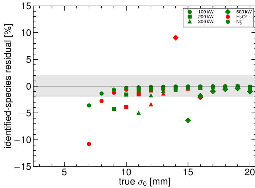
Fig. 16: Aligned extraction identified-species residual versus \sigma_0 at 100, 200, 300 and 500 kW (1 mm I2 grid; B = 0 , 25 kV, 1.6 GeV). Red: \text{H}_2\text{O}^+ . Green: \text{N}_2^+ . The grey band is \pm 2\% . Open markers are wall-clipped families.
