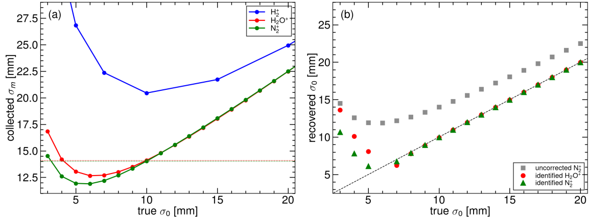
Fig. 15: Aligned extraction, 100 kW, 25 kV, B = 0 , 1.6 GeV. (a) Collected \sigma_m versus true \sigma_0 on the 1 mm I2 grid. Dotted lines are the \text{H}_2\text{O}^+ and \text{N}_2^+ widths of a 10 mm beam (14.11 and 14.03 mm). \text{H}_2^+ is the coarse I1 curve. (b) Leave-one-out invert of the identified \text{H}_2\text{O}^+ or \text{N}_2^+ table on \sigma_0 \geq \sigma_0^* . Grey squares: uncorrected \text{N}_2^+ \sigma_m .
