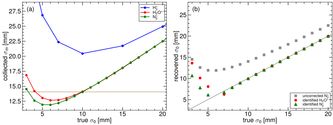
Fig. 14: Aligned extraction, 100 kW, 25 kV, B = 0 , 1.6 GeV. (a) Collected \sigma_m versus true \sigma_0 on the 1 mm I2 grid. Dotted lines are the \text{H}_2\text{O}^+ and \text{N}_2^+ widths of a 10 mm beam (14.11 and 14.03 mm). \text{H}_2^+ is the coarse I1 curve. (b) Leave-one-out invert of the identified \text{H}_2\text{O}^+ or \text{N}_2^+ table on \sigma_0 \geq \sigma_0^* . Grey squares: uncorrected \text{N}_2^+ \sigma_m .
