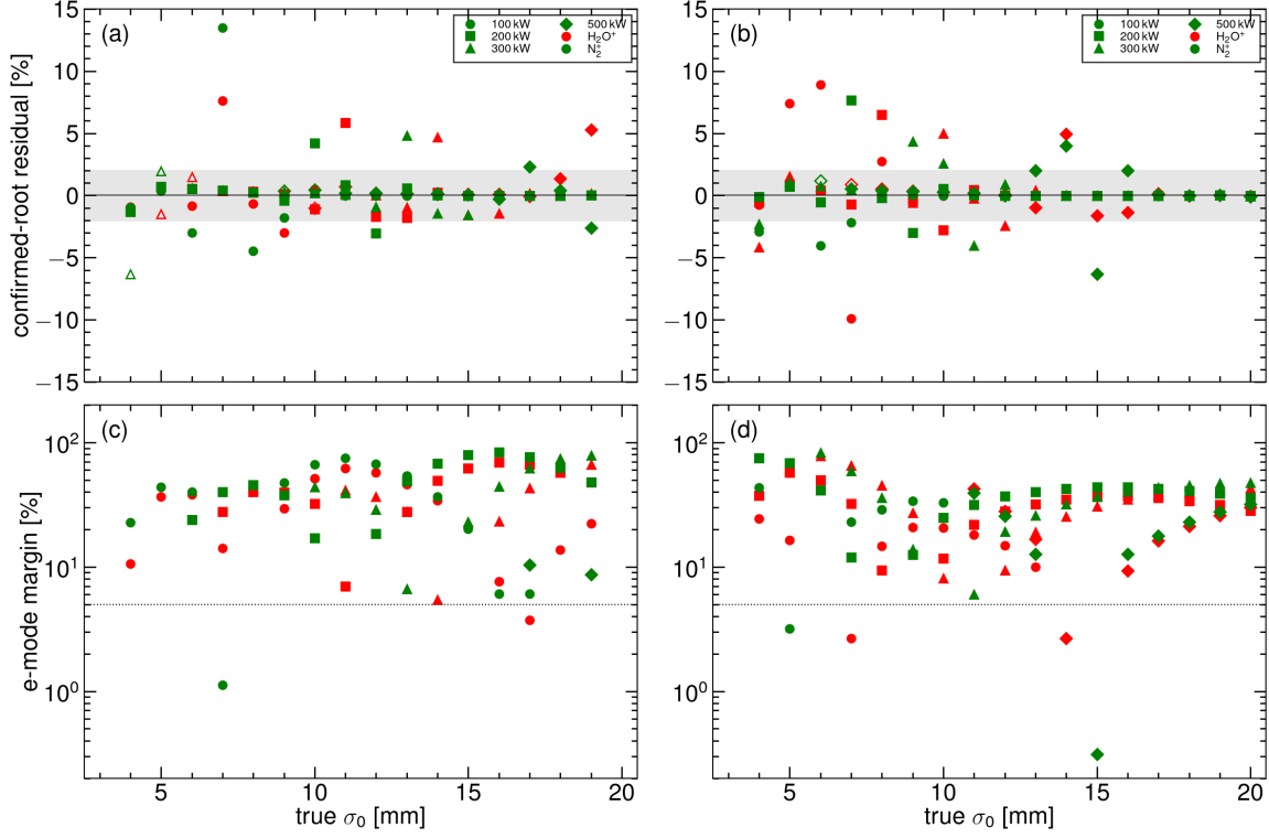
Fig. 14: (a, b) Residual of the root confirmed by the B = 0 electron width versus true \sigma_0 (leave-one-out, grid interior, ions inside the cage) at injection and aligned extraction, 100–500 kW. Red: \text{H}_2\text{O}^+ . Green: \text{N}_2^+ . Open markers are collected above 40 mm. The grey band is \pm 2\% ; the few-percent points are within one step of the fold. (c, d) Electron margin |T_e(\sigma_S) - T_e(\sigma_L)|/\sigma_e at the points with two roots inside the tables; the dotted line is 5%.
