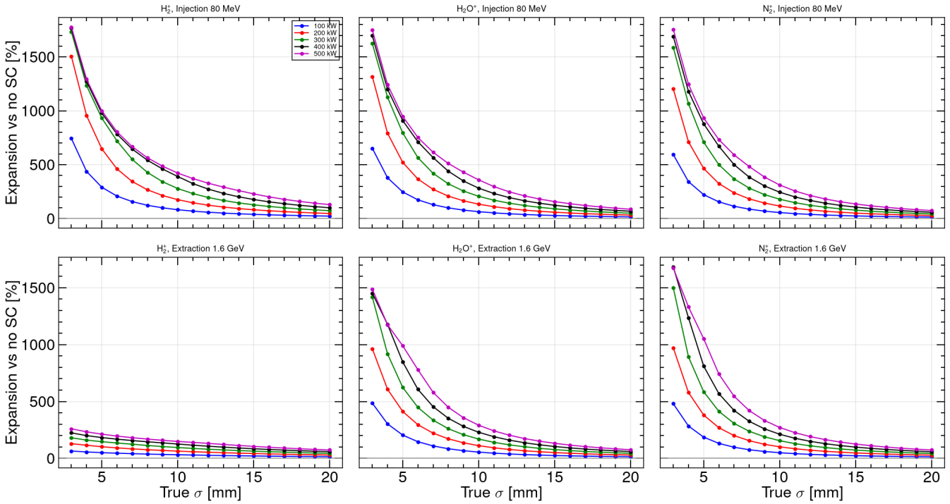
Figure 3. Expansion vs true \sigma_x at 0.1 T for 100–500 kW. Smaller beams and higher power give dramatically larger expansion. On the v1 as-run extraction timing, injection looked worse than extraction for H_2^+ ; after the v2 alignment, extraction H_2^+ is larger than the v1 table (see §3).
